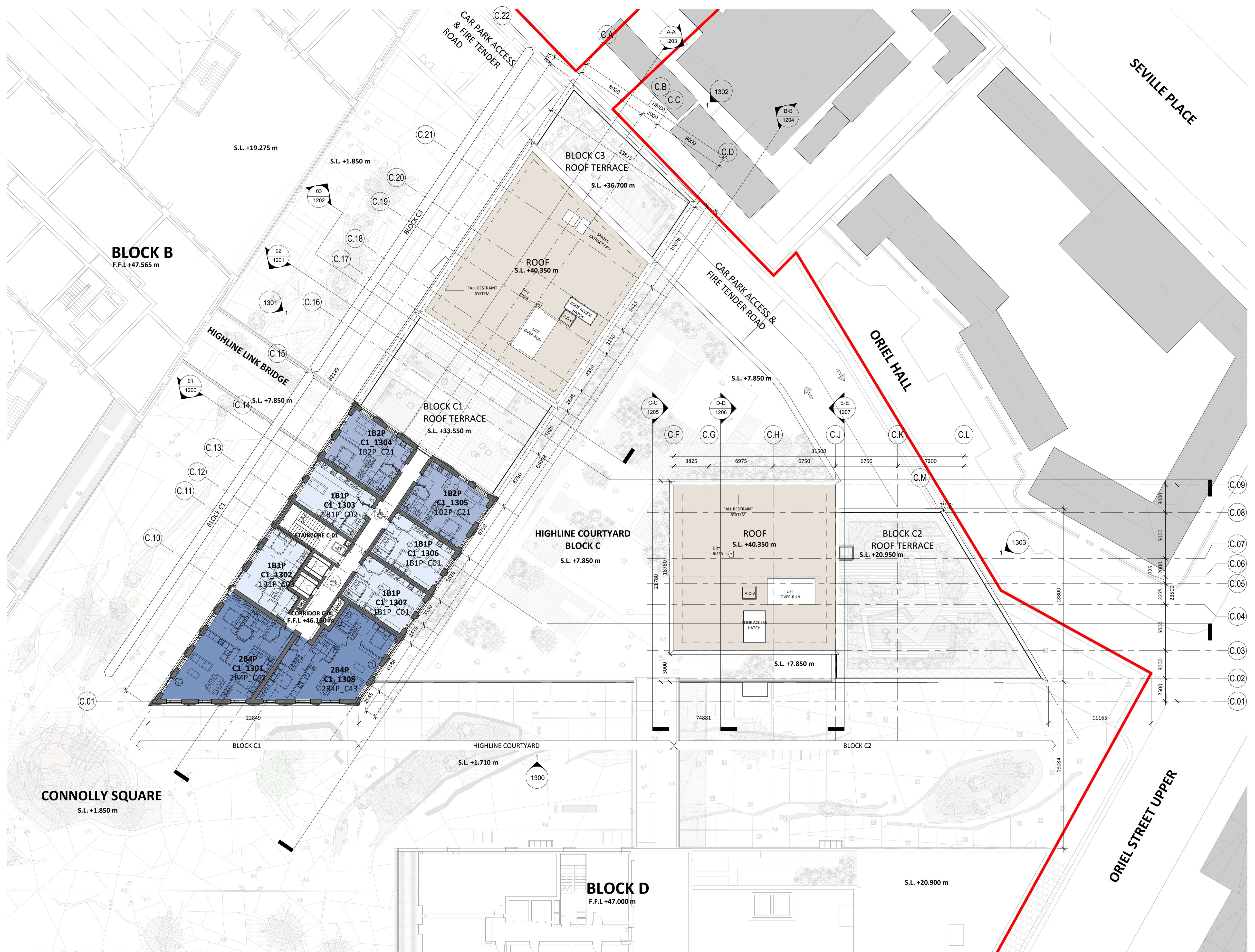
1 BLOCK C PLAN_LEVEL 13 1 : 200
